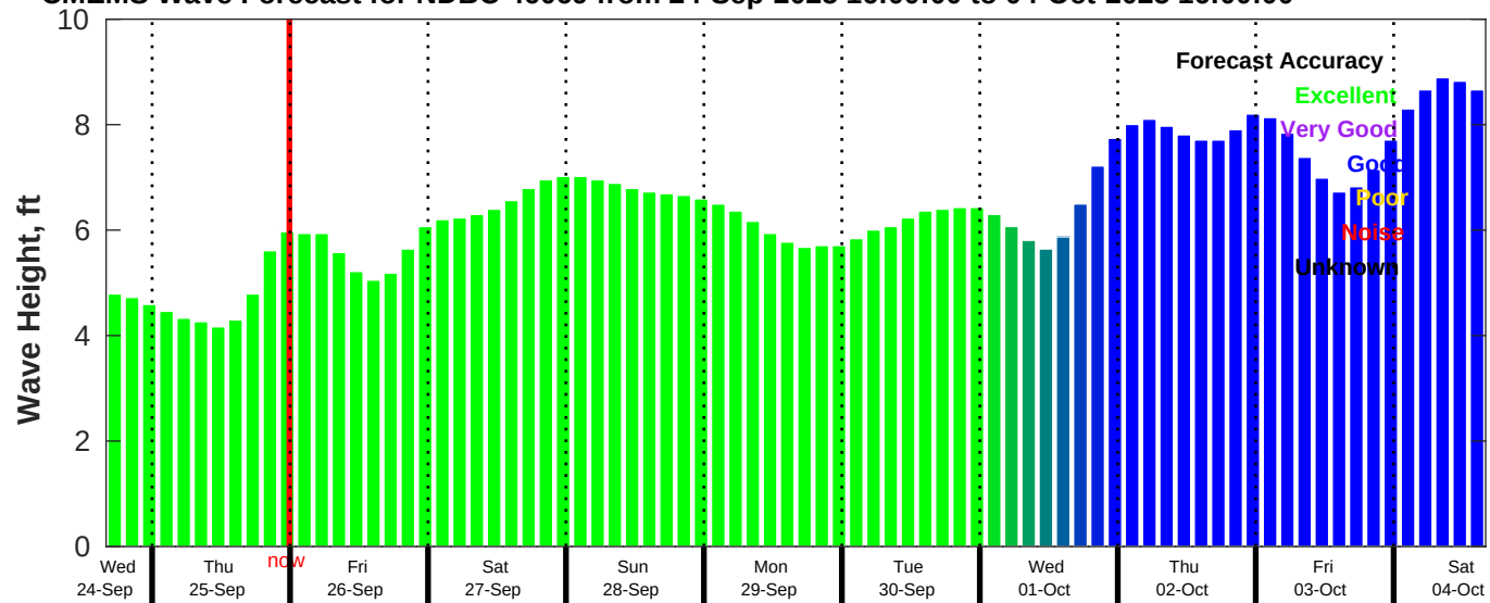
CMEMS Wave Forecast for NDBC 46069 from 24-Sep-2025 16:00:00 to 04-Oct-2025 16:00:00
