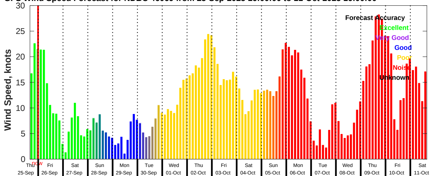
GFS Wind Speed Forecast for NDBC 46069 from 25-Sep-2025 16:00:00 to 11-Oct-2025 16:00:00
