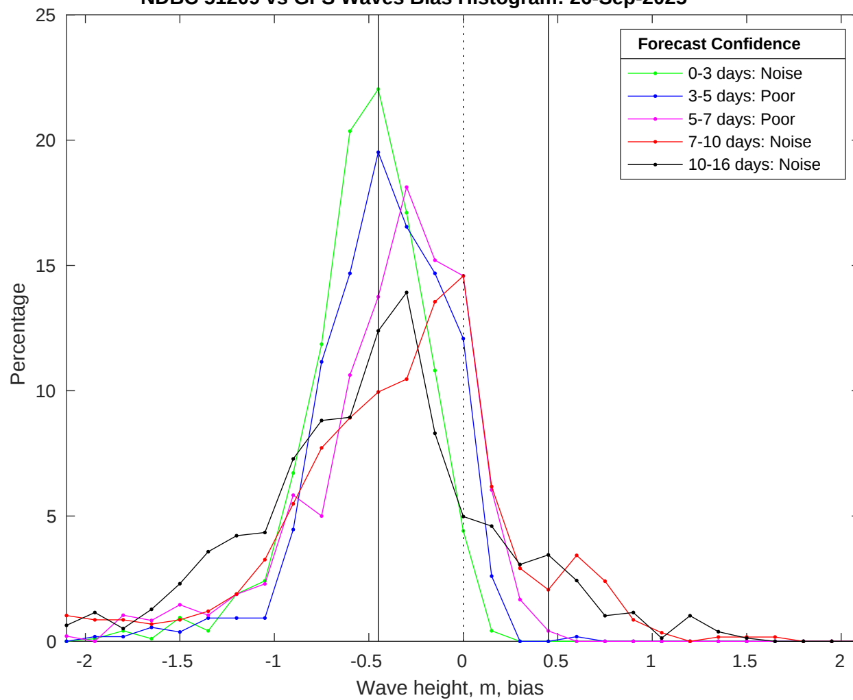
NDBC 51209 vs GFS Waves Bias Histogram: 26-Sep-2025
