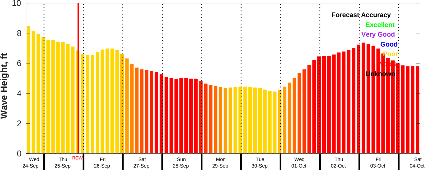
CMEMS Wave Forecast for NDBC 51209 from 24-Sep-2025 13:00:00 to 04-Oct-2025 13:00:00
