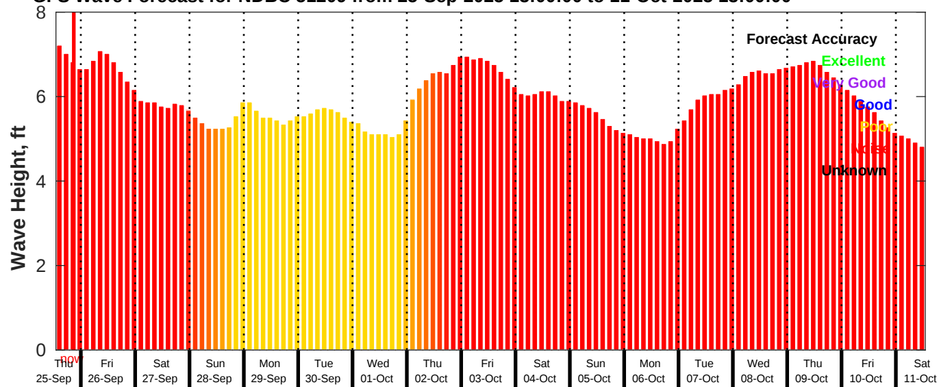
GFS Wave Forecast for NDBC 51209 from 25-Sep-2025 13:00:00 to 11-Oct-2025 13:00:00
