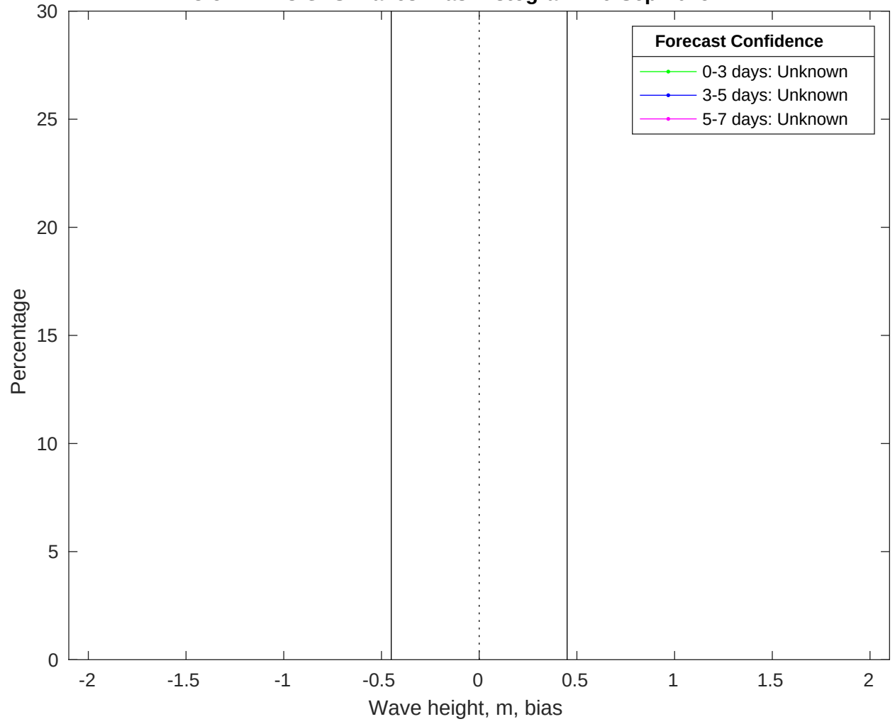
NDBC 51211 vs GFS Waves Bias Histogram: 26-Sep-2025
