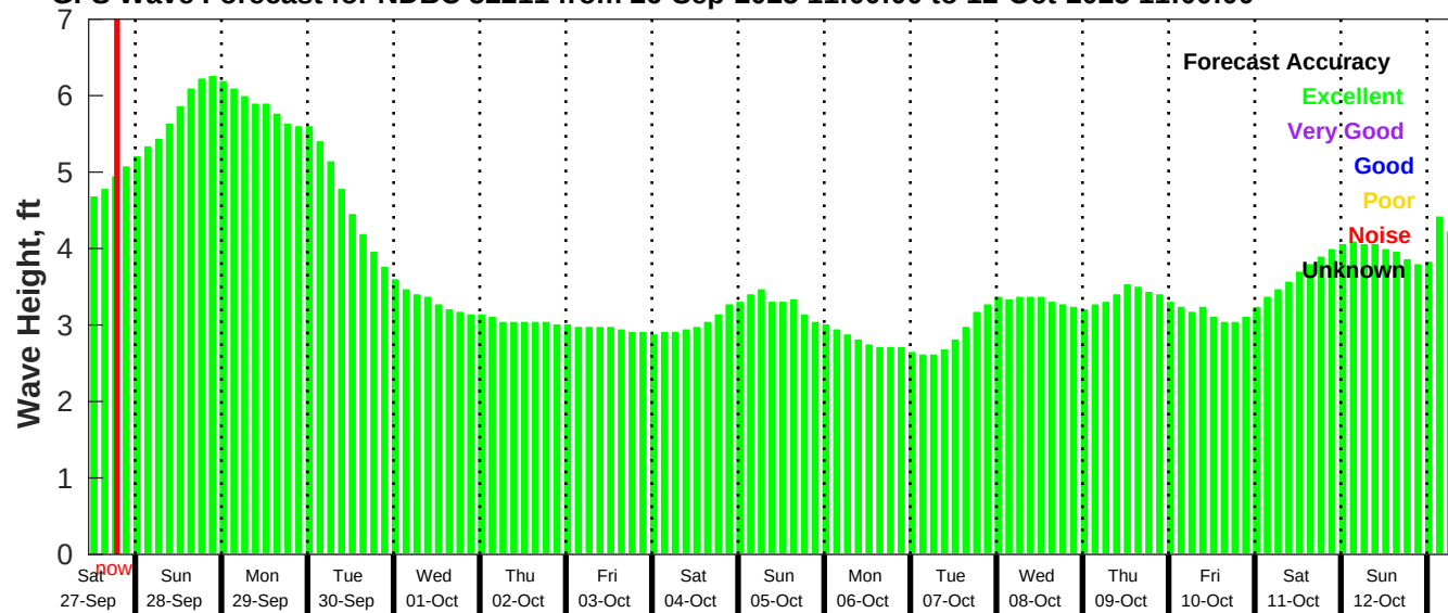
GFS Wave Forecast for NDBC 52211 from 26-Sep-2025 11:00:00 to 12-Oct-2025 11:00:00
