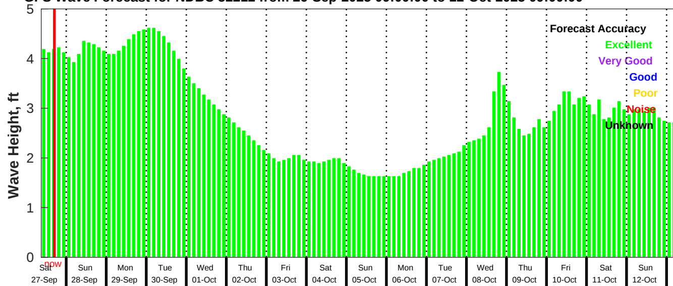
GFS Wave Forecast for NDBC 52212 from 26-Sep-2025 09:00:00 to 12-Oct-2025 09:00:00
