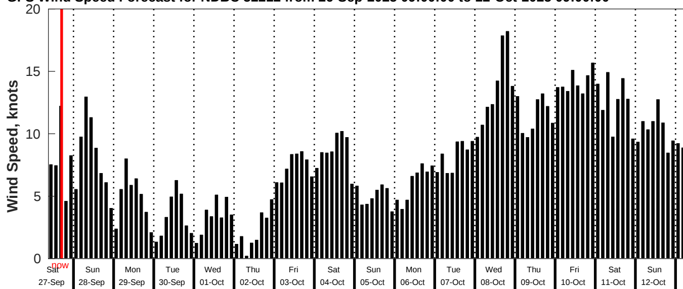
GFS Wind Speed Forecast for NDBC 52212 from 26-Sep-2025 09:00:00 to 12-Oct-2025 09:00:00
