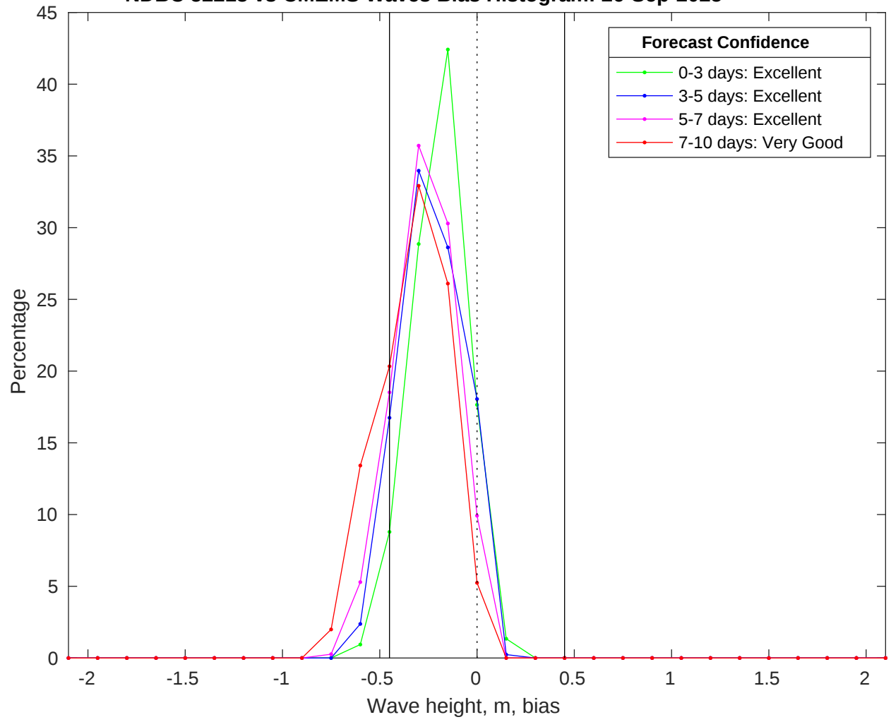
NDBC 52213 vs CMEMS Waves Bias Histogram: 26-Sep-2025
