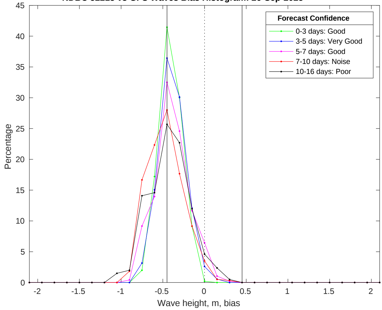
NDBC 52213 vs GFS Waves Bias Histogram: 26-Sep-2025
