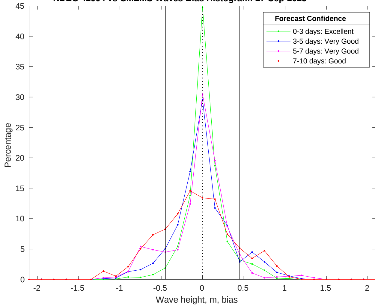
NDBC 41004 vs CMEMS Waves Bias Histogram: 27-Sep-2025
