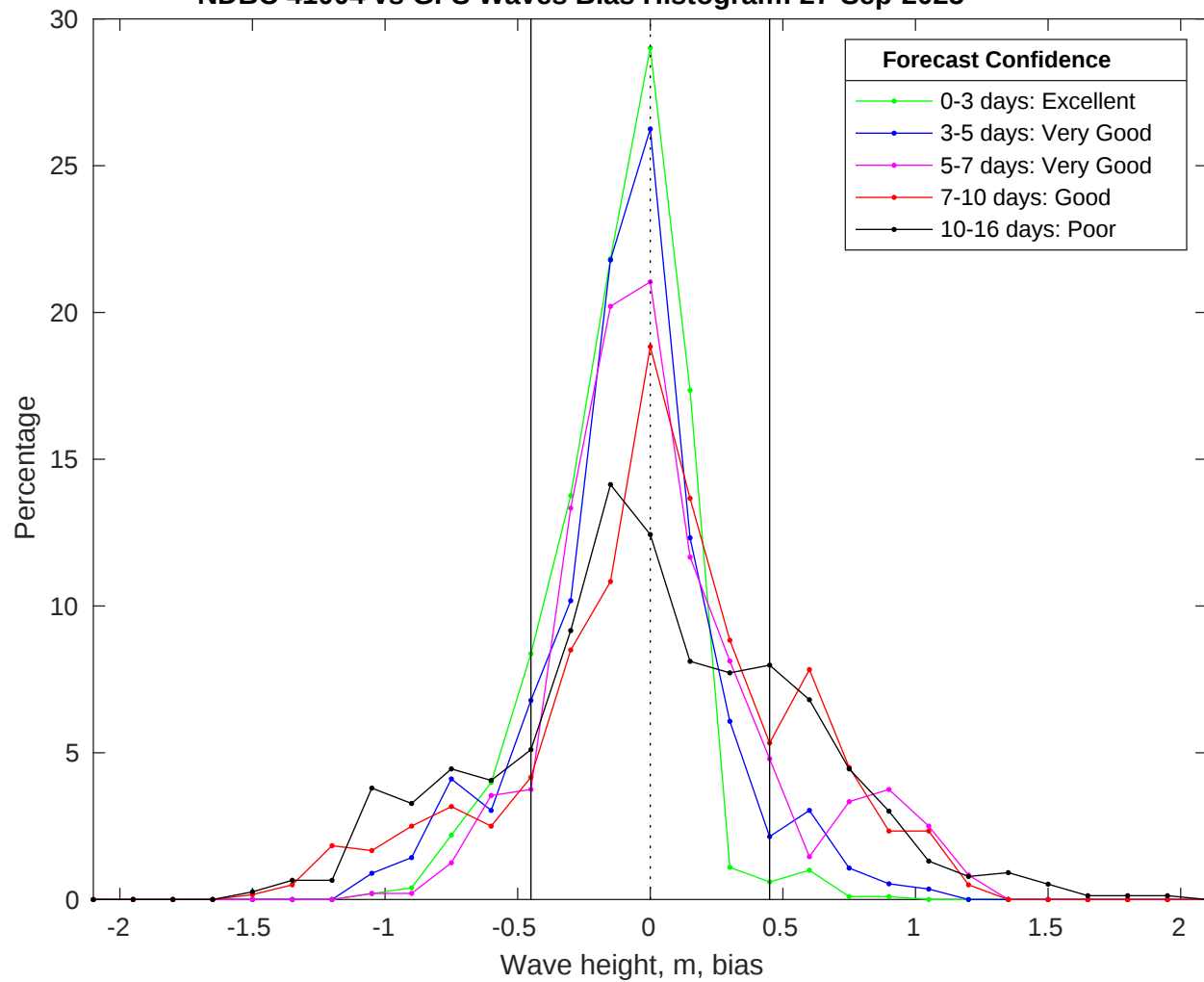
NDBC 41004 vs GFS Waves Bias Histogram: 27-Sep-2025
