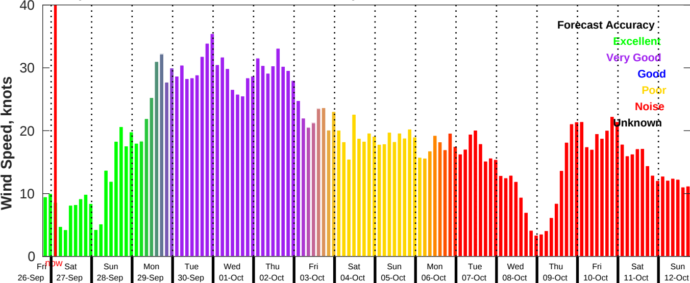
GFS Wind Speed Forecast for NDBC 41004 from 26-Sep-2025 19:00:00 to 12-Oct-2025 19:00:00
