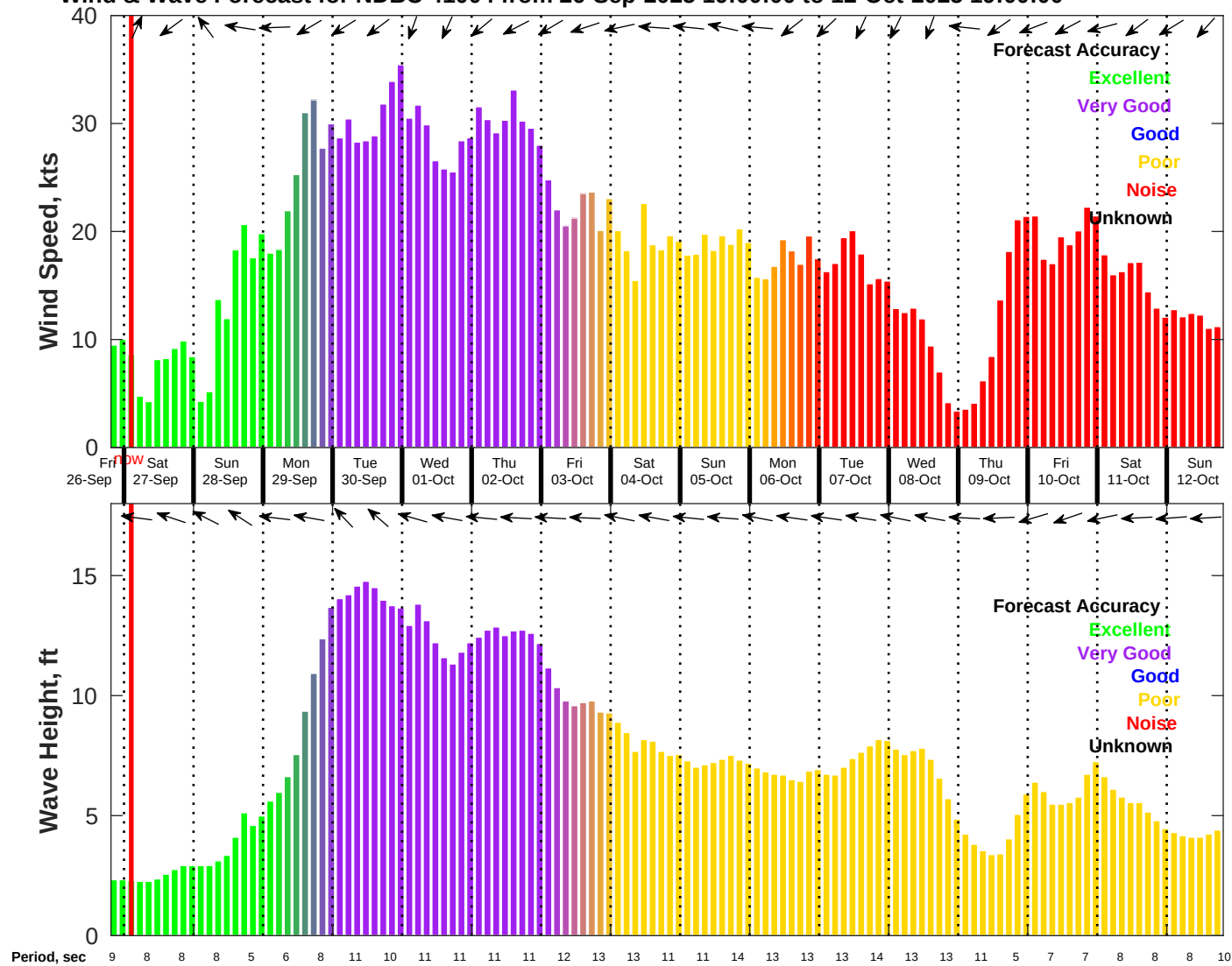
Wind & Wave Forecast for NDBC 41004 from 26-Sep-2025 19:00:00 to 12-Oct-2025 19:00:00
