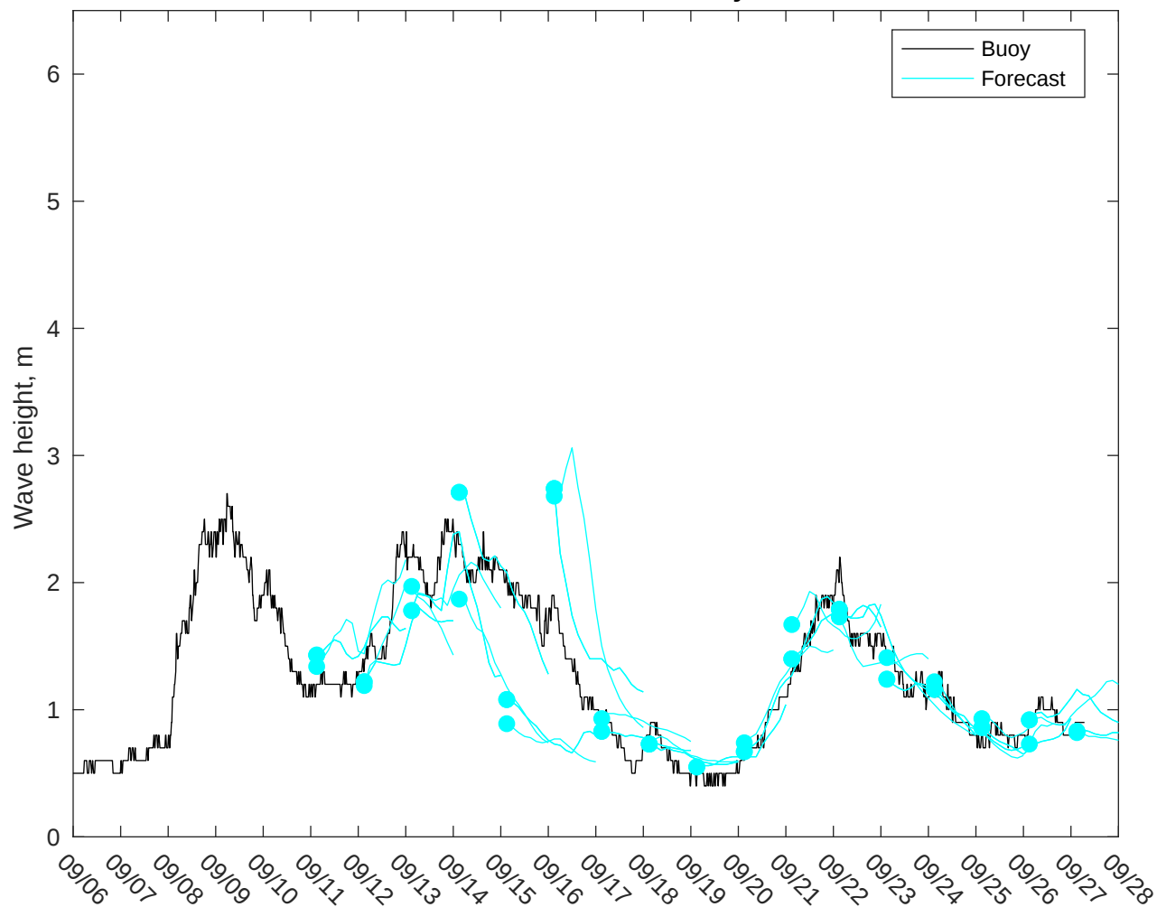
NDBC 41013 vs CMEMS Waves: 5 to 7 day forecast
