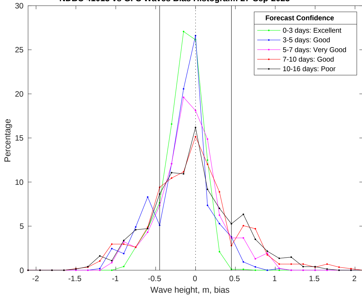
NDBC 41013 vs GFS Waves Bias Histogram: 27-Sep-2025
