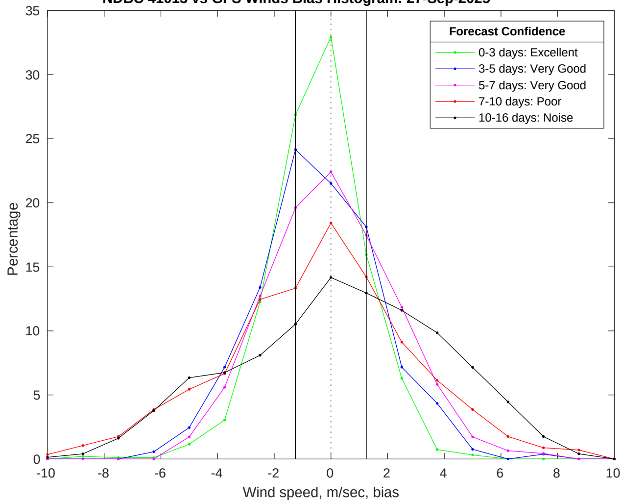
NDBC 41013 vs GFS Winds Bias Histogram: 27-Sep-2025
