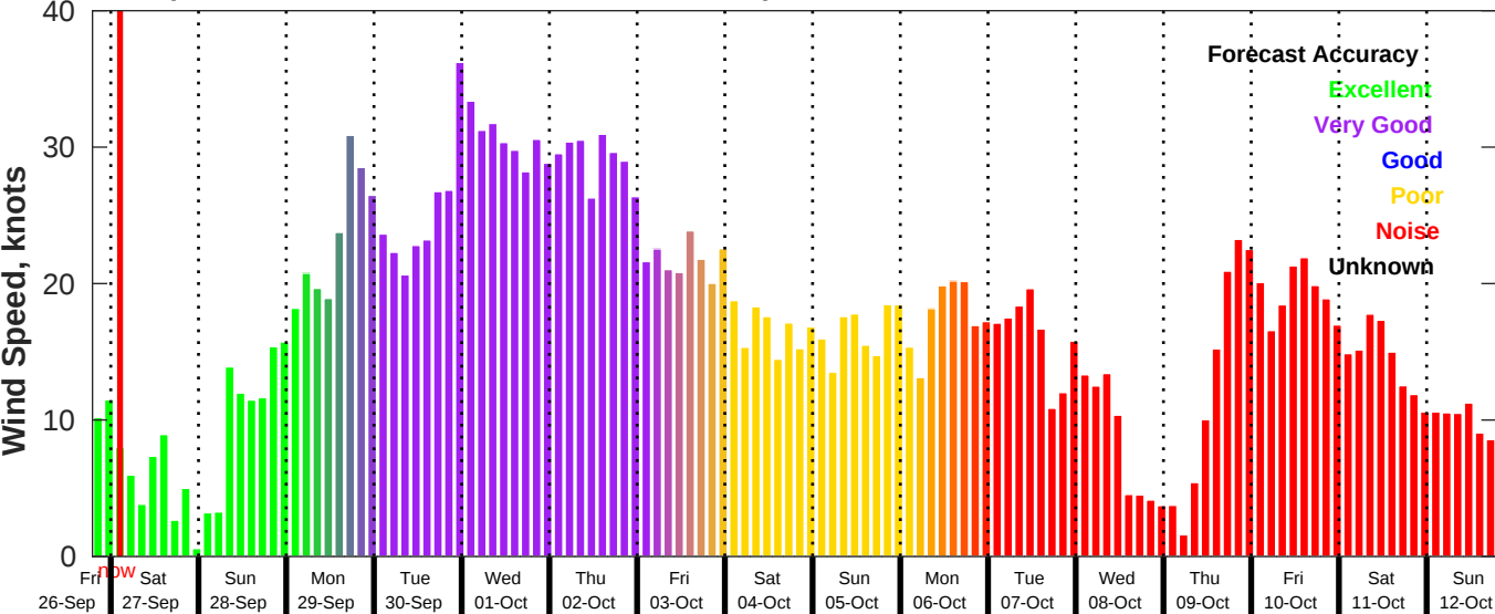
GFS Wind Speed Forecast for NDBC 41013 from 26-Sep-2025 19:00:00 to 12-Oct-2025 19:00:00
