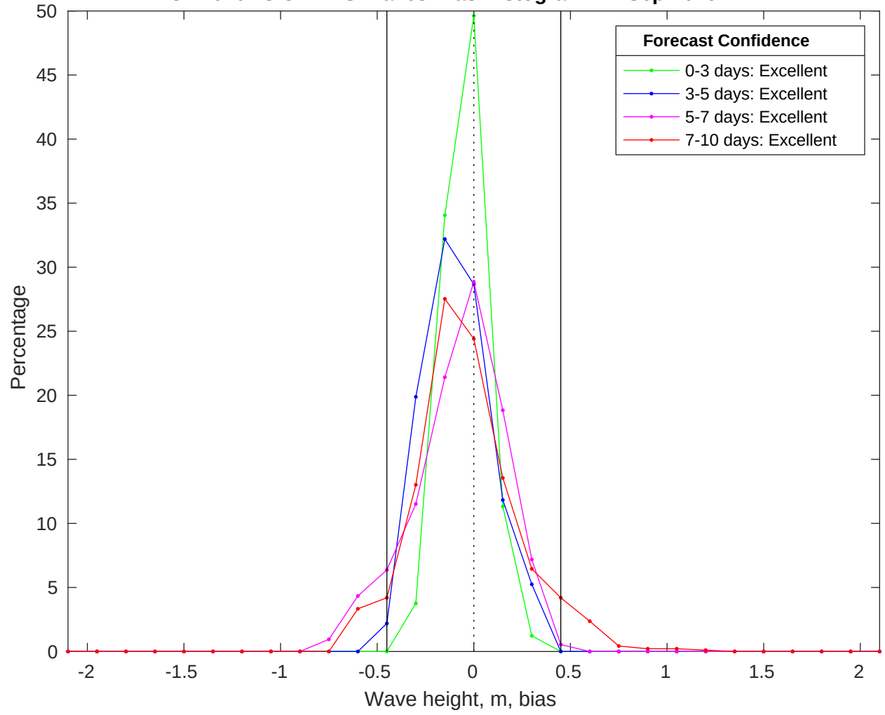
NDBC 41040 vs CMEMS Waves Bias Histogram: 27-Sep-2025
