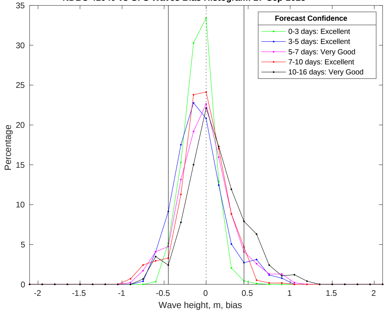
NDBC 41040 vs GFS Waves Bias Histogram: 27-Sep-2025
