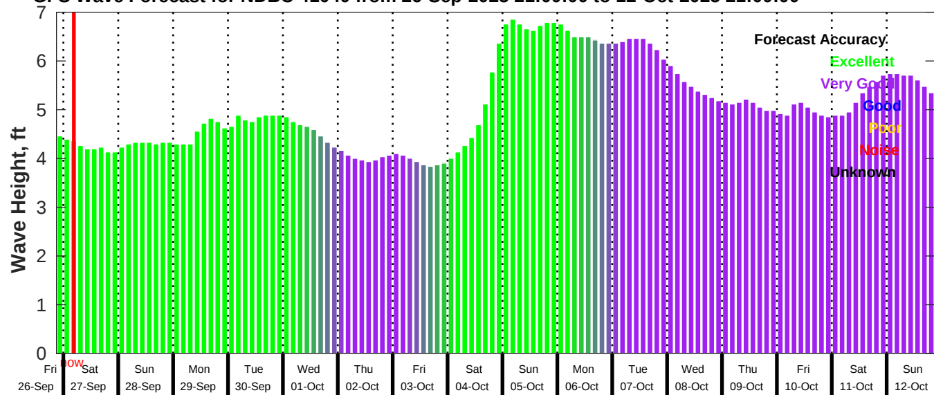
GFS Wave Forecast for NDBC 41040 from 26-Sep-2025 21:00:00 to 12-Oct-2025 21:00:00
