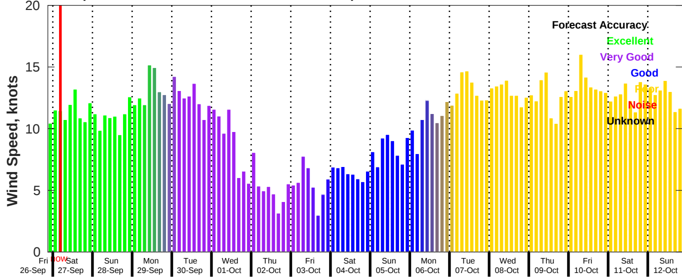
GFS Wind Speed Forecast for NDBC 41040 from 26-Sep-2025 21:00:00 to 12-Oct-2025 21:00:00
