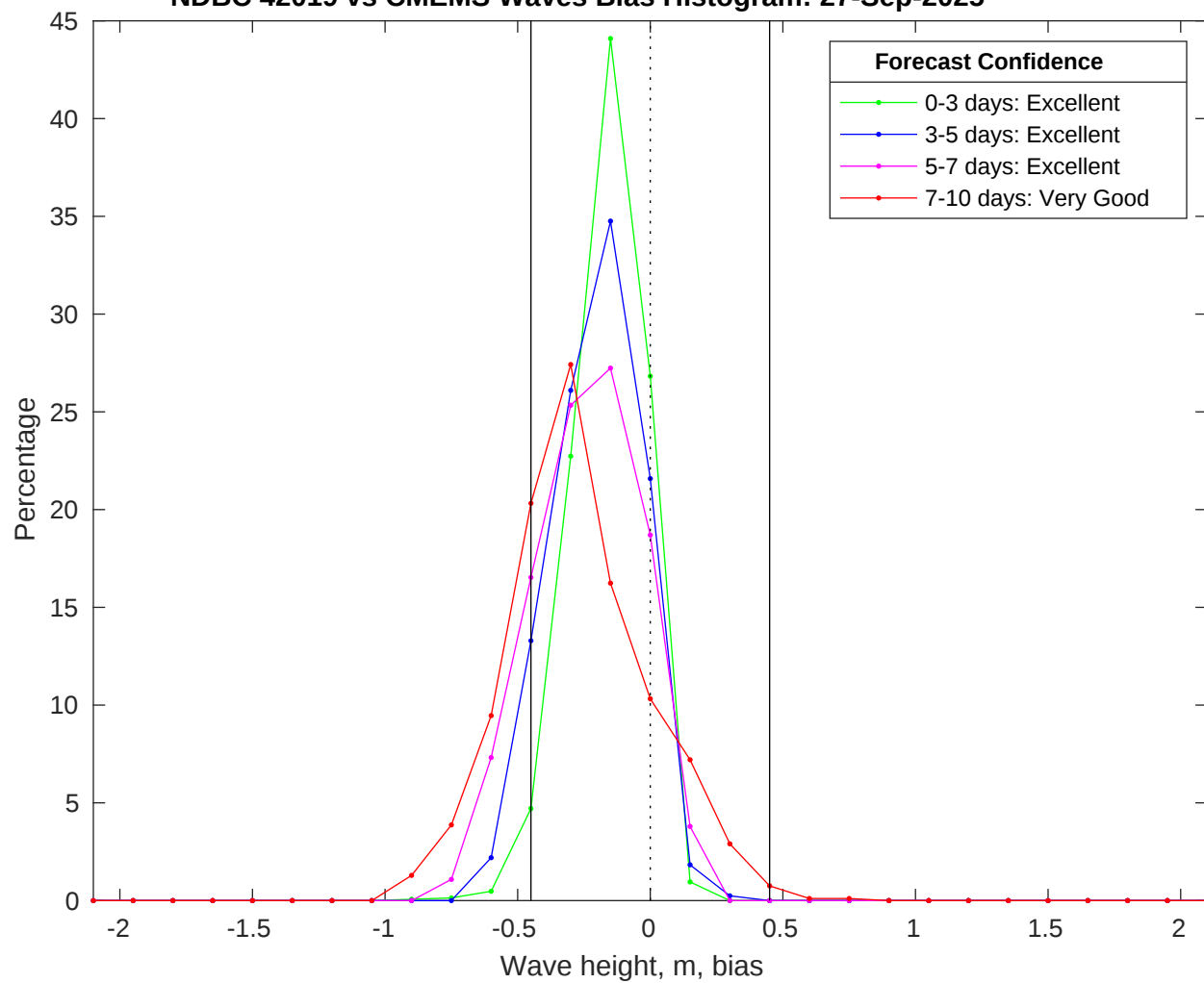
NDBC 42019 vs CMEMS Waves Bias Histogram: 27-Sep-2025
