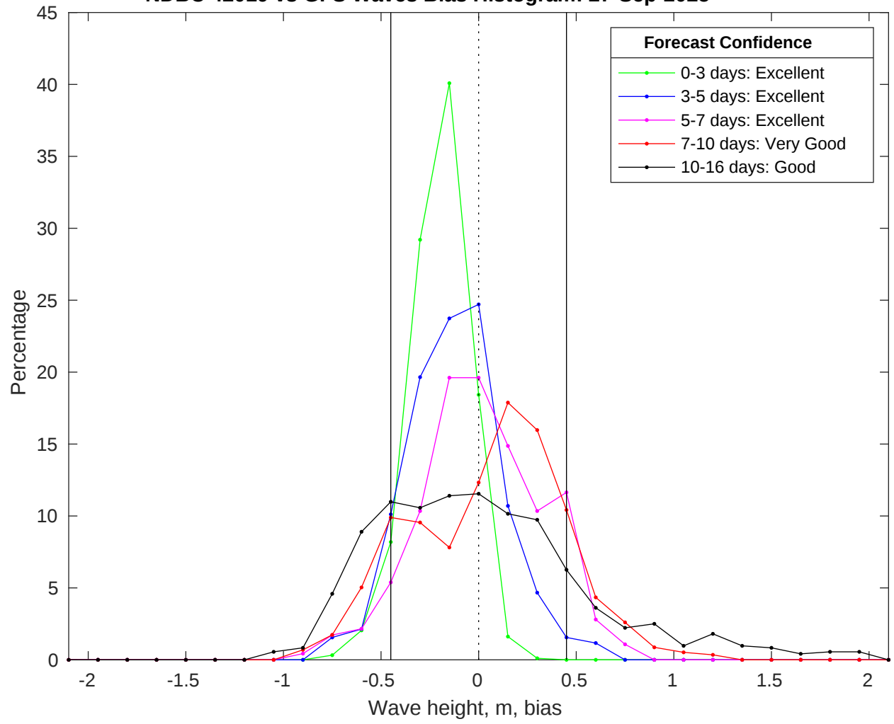
NDBC 42019 vs GFS Waves Bias Histogram: 27-Sep-2025
