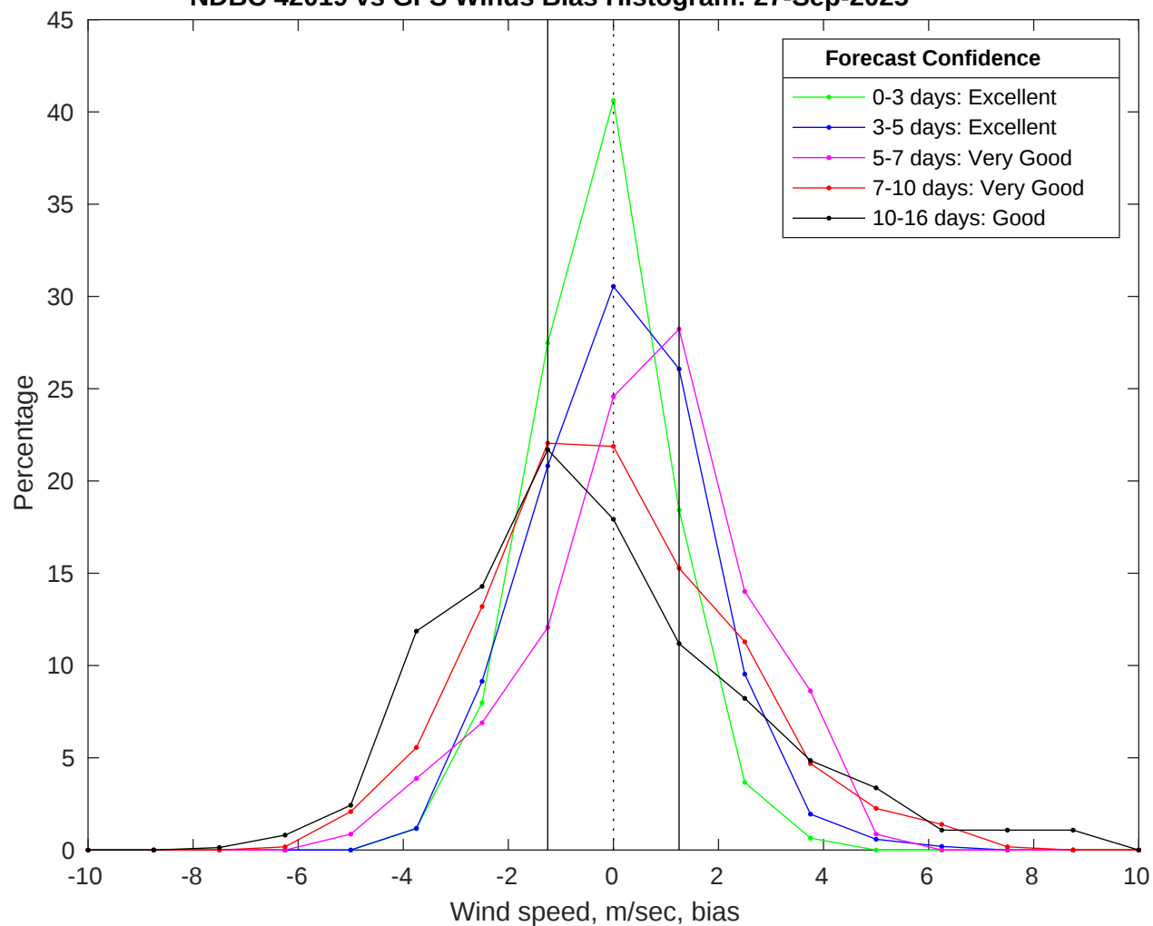
NDBC 42019 vs GFS Winds Bias Histogram: 27-Sep-2025
