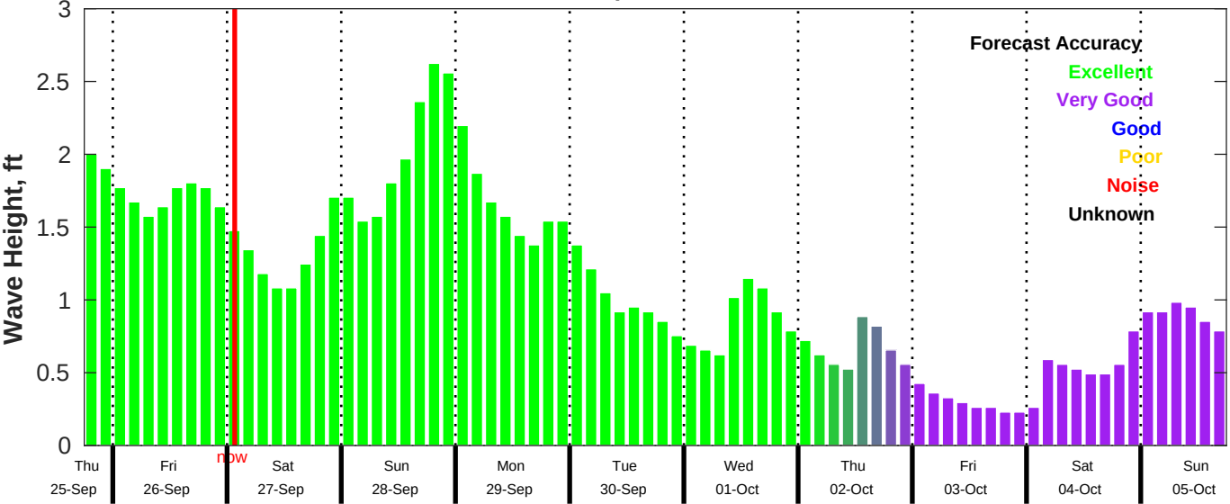
CMEMS Wave Forecast for NDBC 42019 from 25-Sep-2025 18:00:00 to 05-Oct-2025 18:00:00
