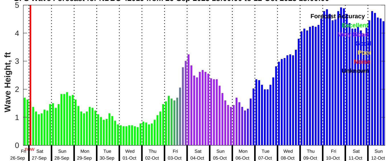
GFS Wave Forecast for NDBC 42019 from 26-Sep-2025 18:00:00 to 12-Oct-2025 18:00:00
