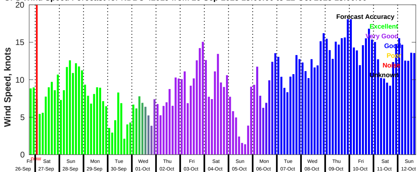
GFS Wind Speed Forecast for NDBC 42019 from 26-Sep-2025 18:00:00 to 12-Oct-2025 18:00:00
