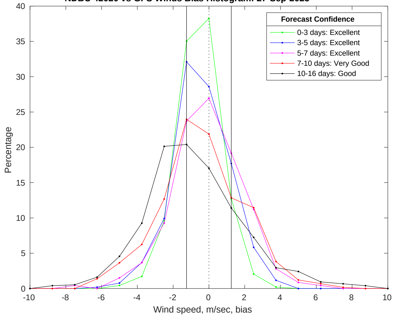
NDBC 42020 vs GFS Winds Bias Histogram: 27-Sep-2025
