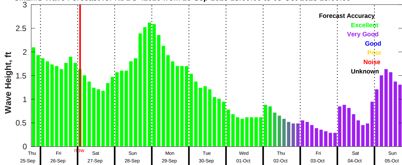
CMEMS Wave Forecast for NDBC 42020 from 25-Sep-2025 18:00:00 to 05-Oct-2025 18:00:00
