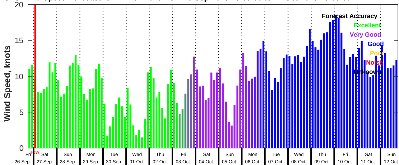
GFS Wind Speed Forecast for NDBC 42020 from 26-Sep-2025 18:00:00 to 12-Oct-2025 18:00:00
