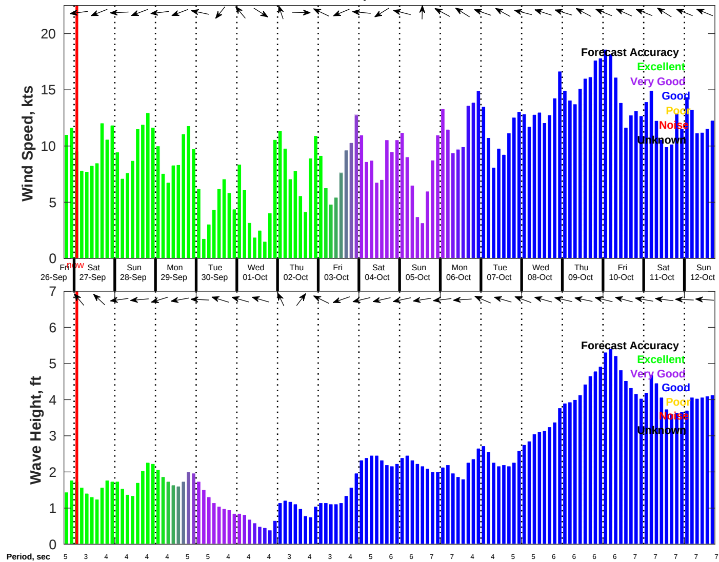
Wind & Wave Forecast for NDBC 42020 from 26-Sep-2025 18:00:00 to 12-Oct-2025 18:00:00
