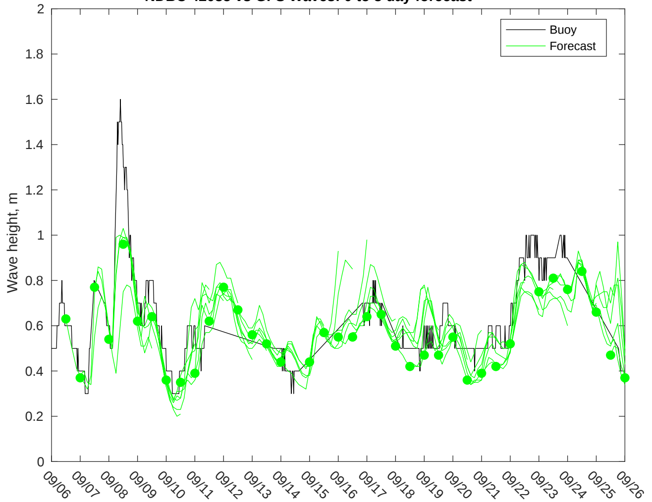
NDBC 42035 vs GFS Waves: 0 to 3 day forecast
