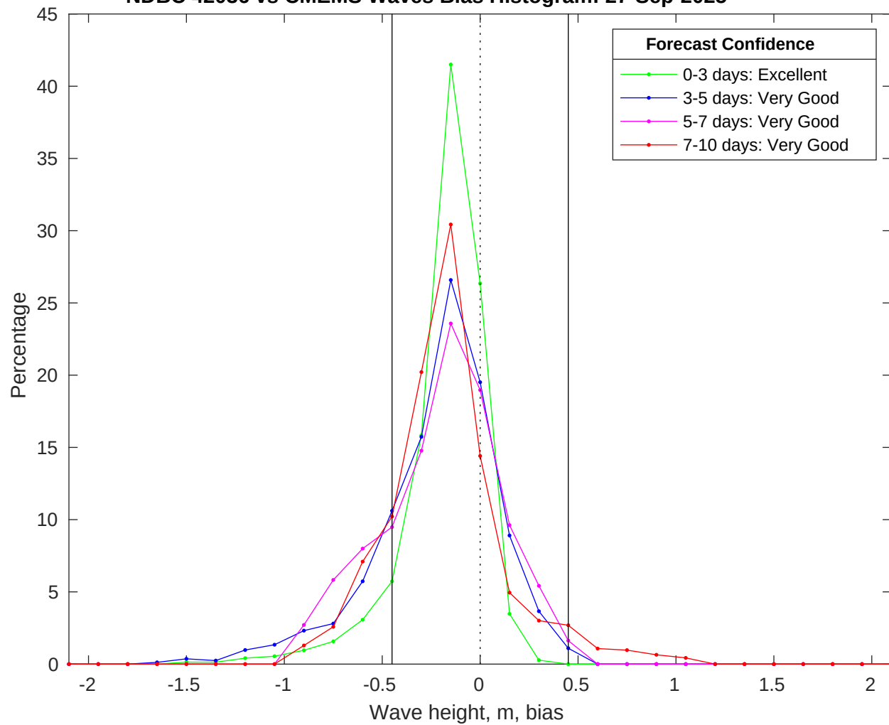
NDBC 42036 vs CMEMS Waves Bias Histogram: 27-Sep-2025
