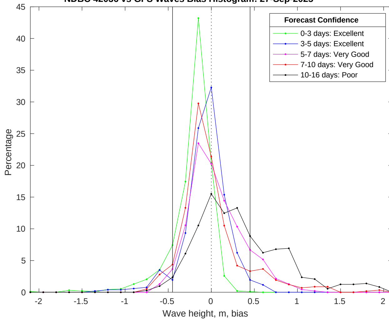
NDBC 42036 vs GFS Waves Bias Histogram: 27-Sep-2025
