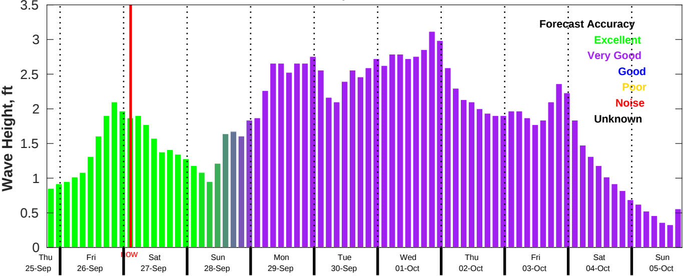
CMEMS Wave Forecast for NDBC 42036 from 25-Sep-2025 19:00:00 to 05-Oct-2025 19:00:00
