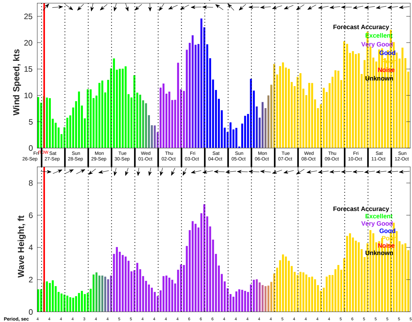
Wind & Wave Forecast for NDBC 42036 from 26-Sep-2025 19:00:00 to 12-Oct-2025 19:00:00
