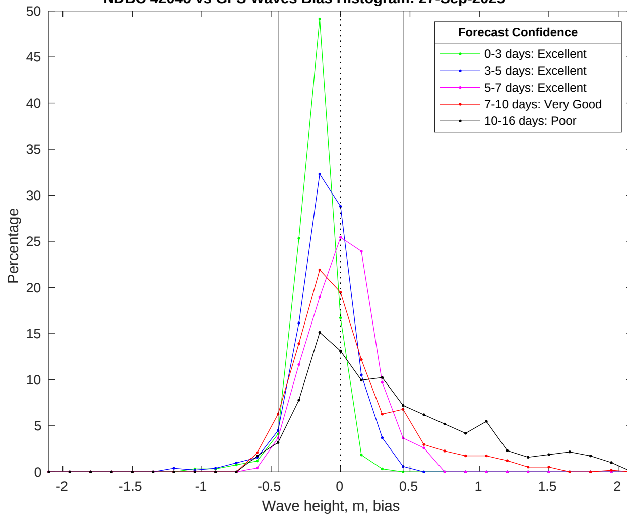
NDBC 42040 vs GFS Waves Bias Histogram: 27-Sep-2025
