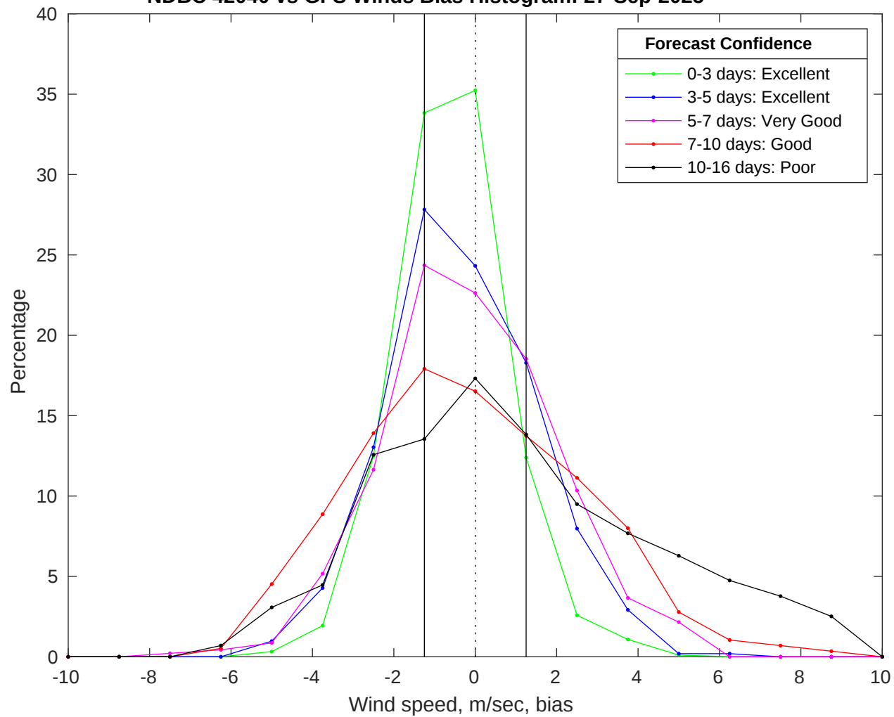
NDBC 42040 vs GFS Winds Bias Histogram: 27-Sep-2025
