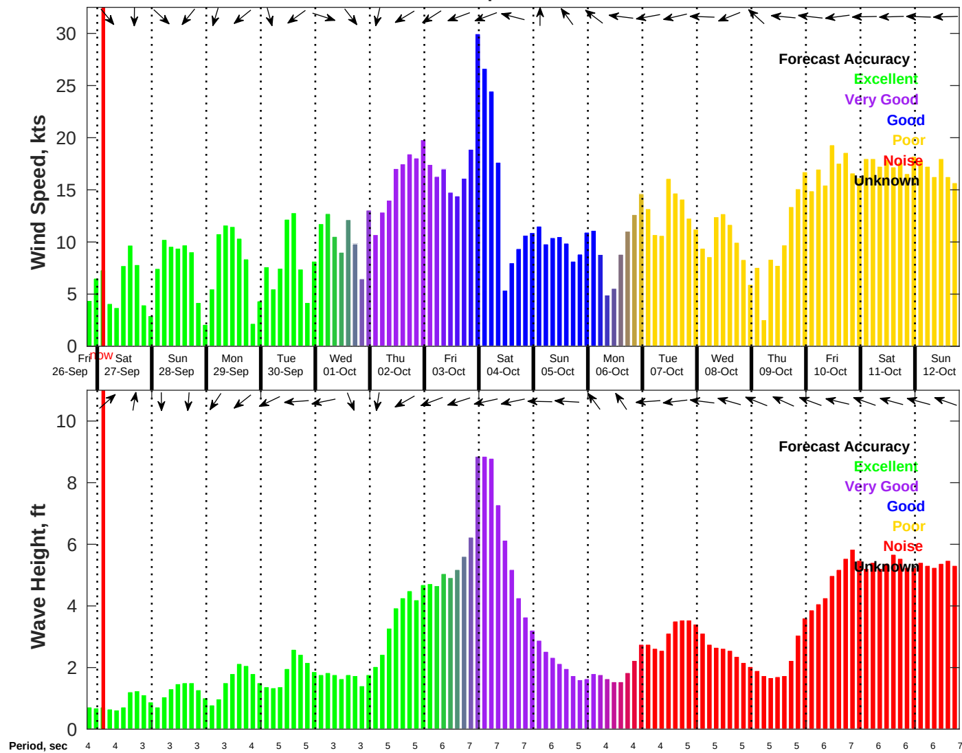
Wind & Wave Forecast for NDBC 42040 from 26-Sep-2025 19:00:00 to 12-Oct-2025 19:00:00
