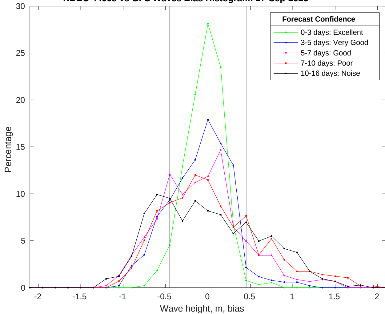
NDBC 44008 vs GFS Waves Bias Histogram: 27-Sep-2025
