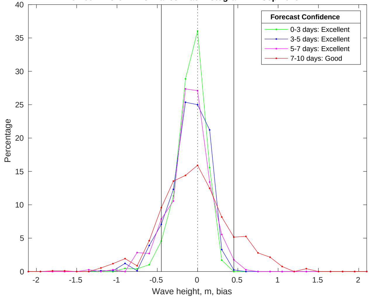
NDBC 46011 vs CMEMS Waves Bias Histogram: 27-Sep-2025
