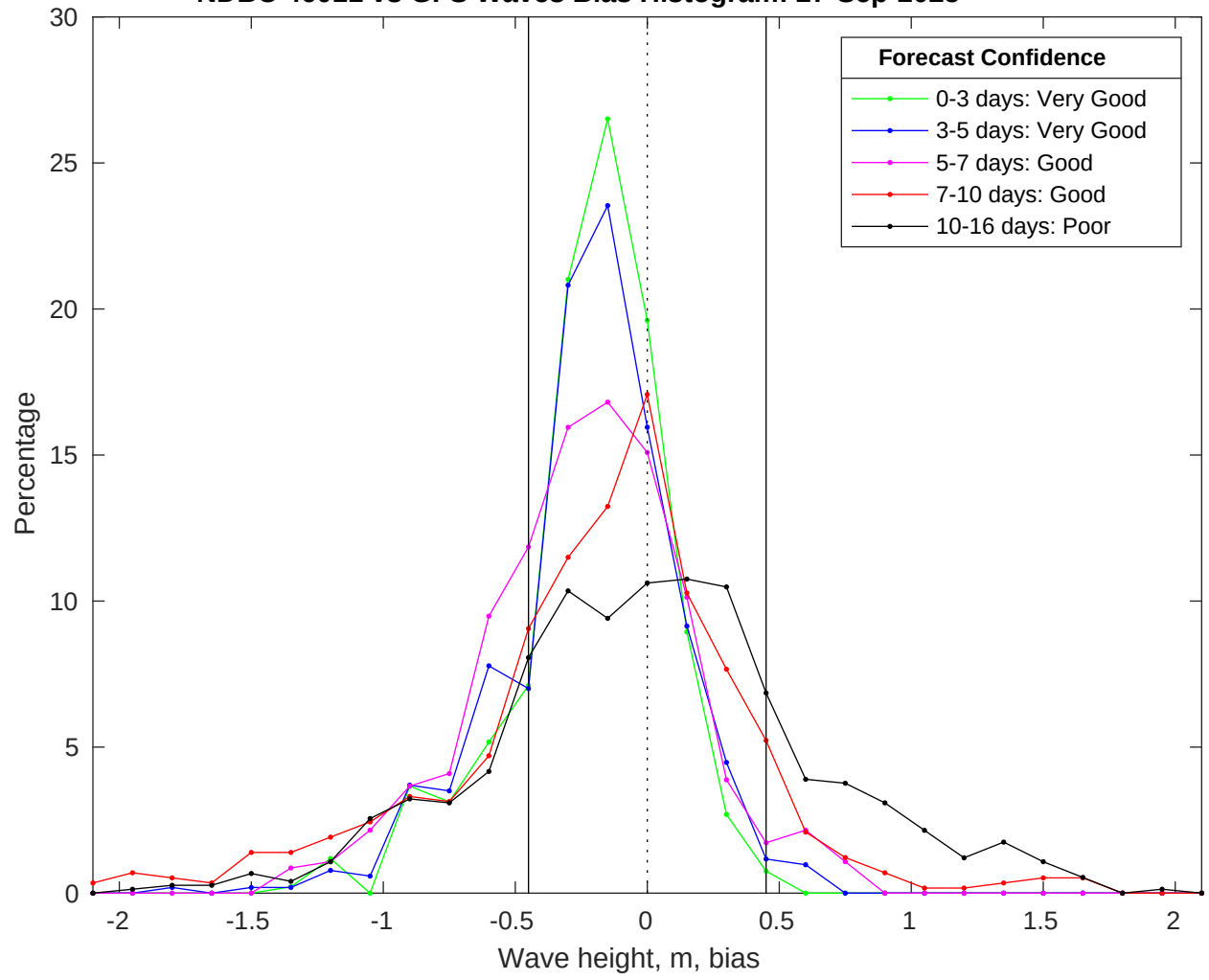
NDBC 46011 vs GFS Waves Bias Histogram: 27-Sep-2025
