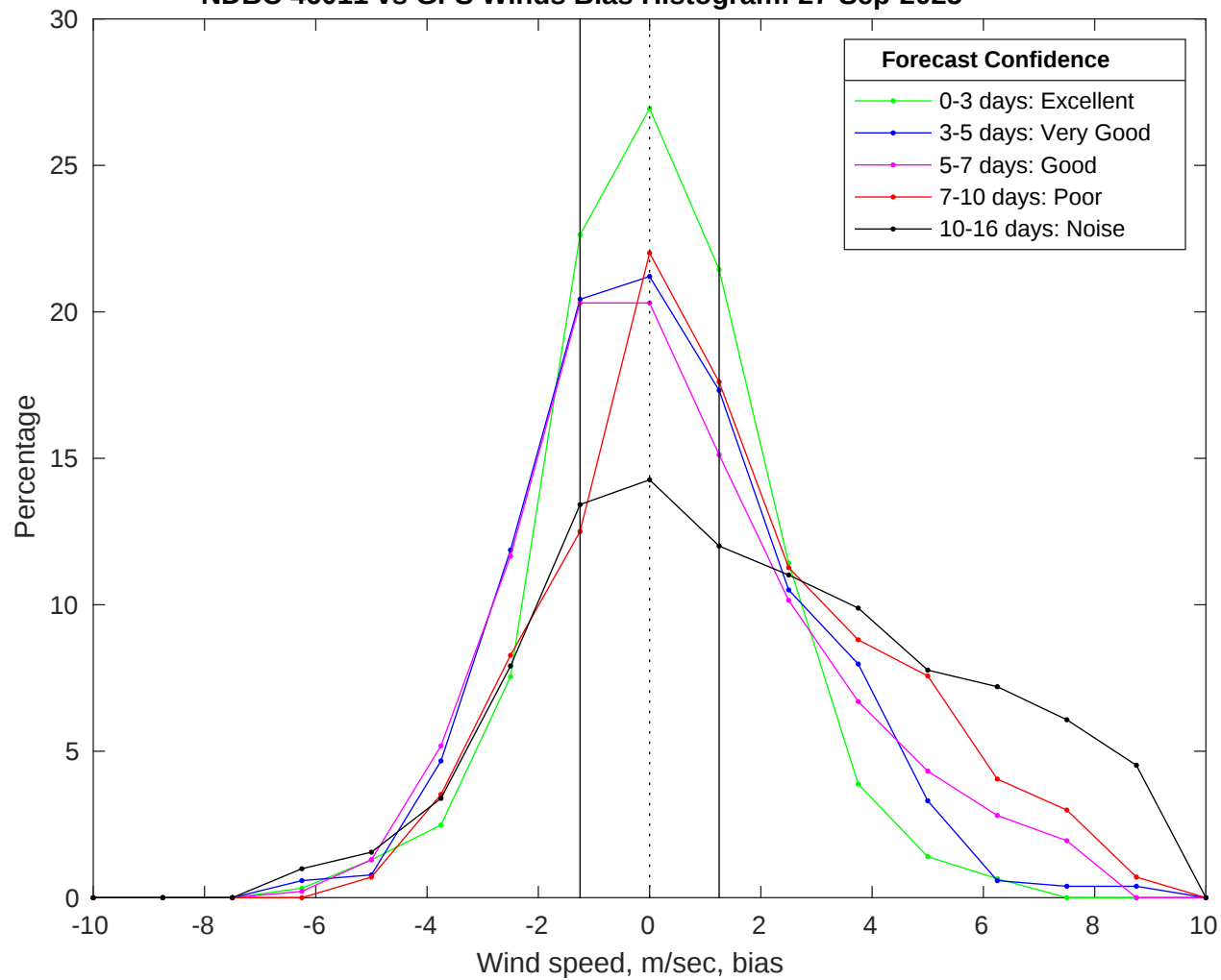
NDBC 46011 vs GFS Winds Bias Histogram: 27-Sep-2025
