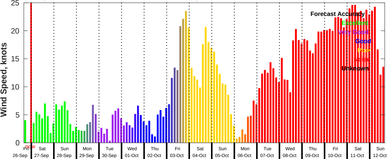
GFS Wind Speed Forecast for NDBC 46011 from 26-Sep-2025 16:00:00 to 12-Oct-2025 16:00:00
