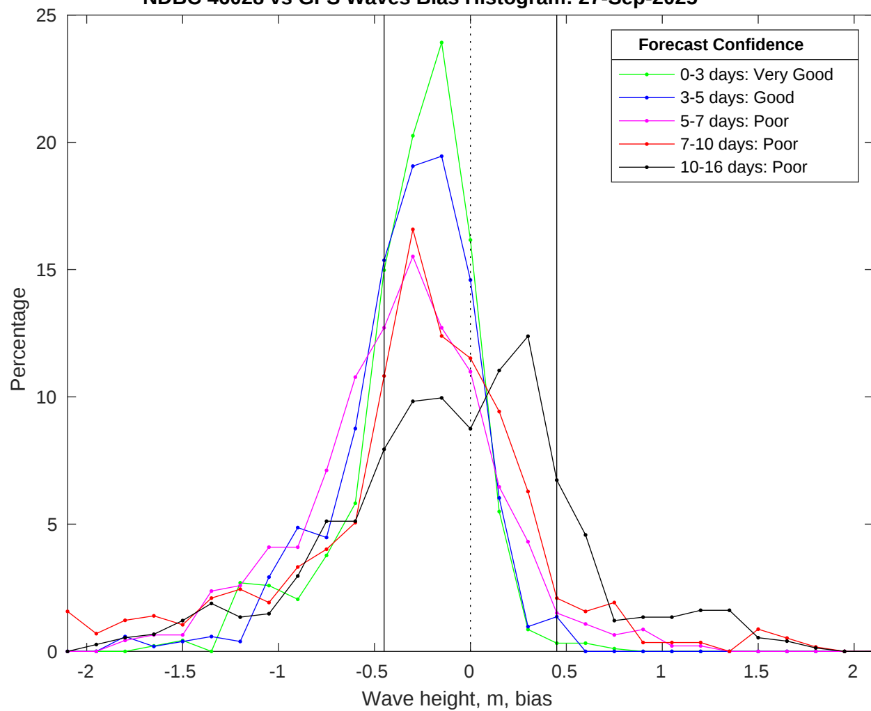
NDBC 46028 vs GFS Waves Bias Histogram: 27-Sep-2025
