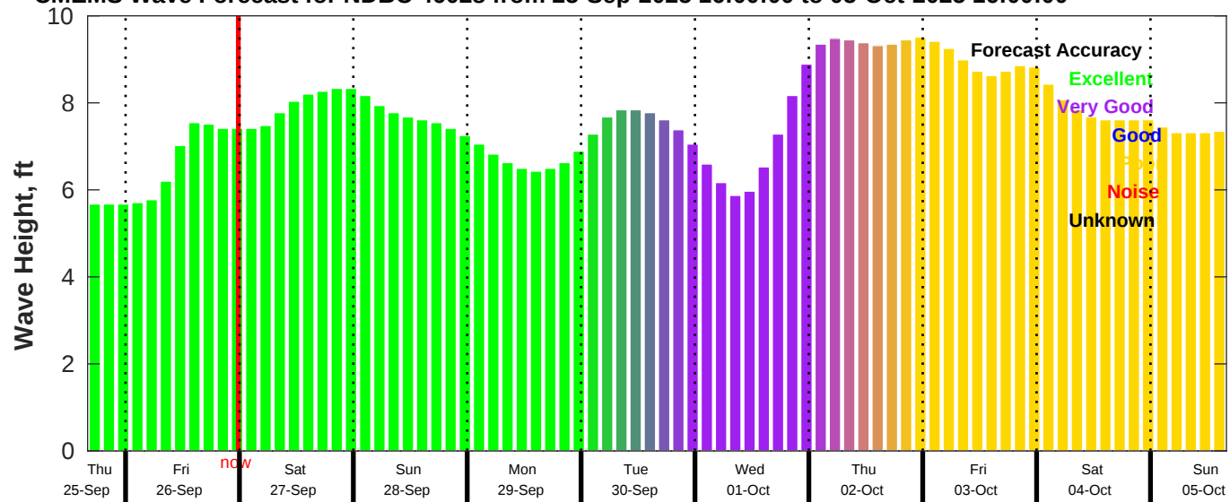
CMEMS Wave Forecast for NDBC 46028 from 25-Sep-2025 16:00:00 to 05-Oct-2025 16:00:00
