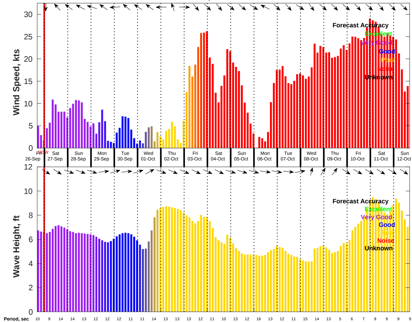
Wind & Wave Forecast for NDBC 46028 from 26-Sep-2025 16:00:00 to 12-Oct-2025 16:00:00
