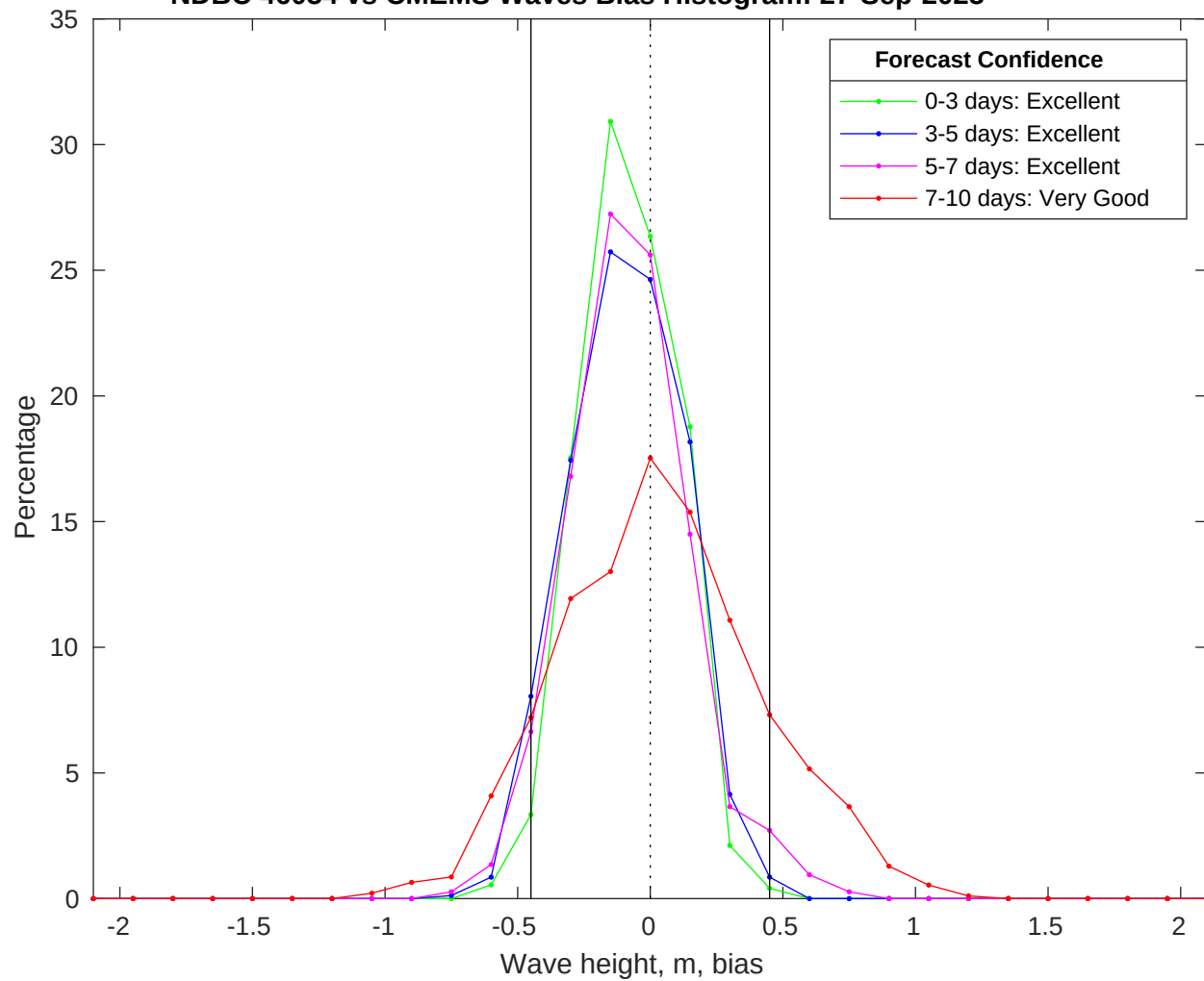
NDBC 46054 vs CMEMS Waves Bias Histogram: 27-Sep-2025
